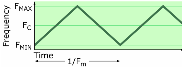
Figure: Output Frequency Modulation Width
