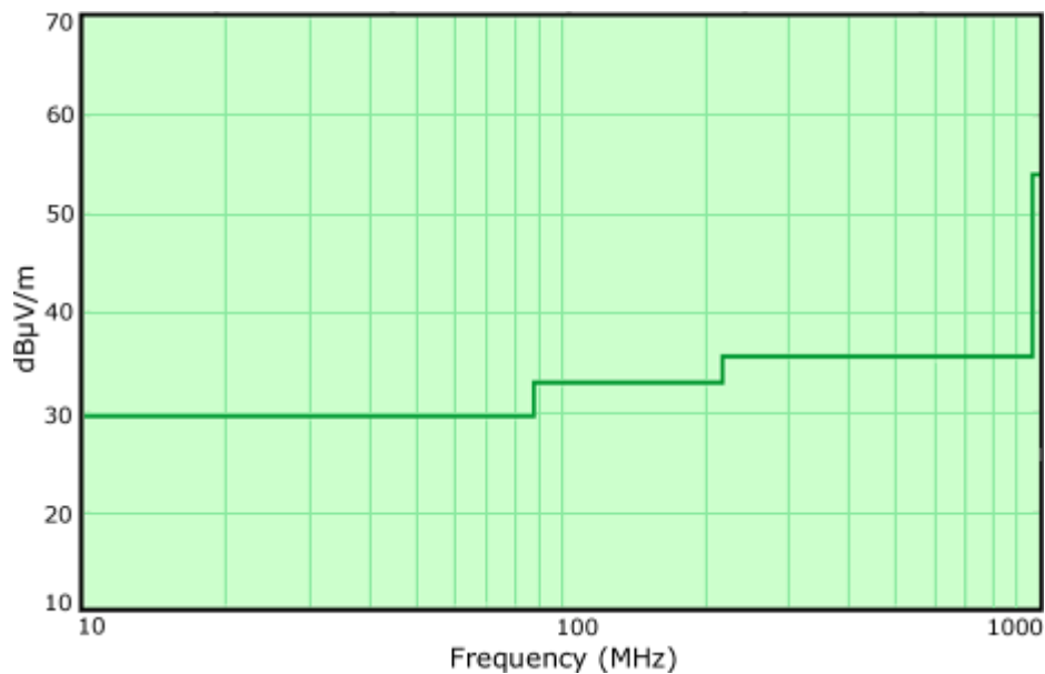
Figure: FCC Class B Peak Emissions
