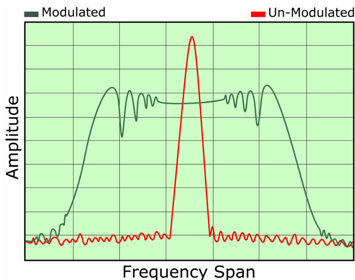
Figure: EMI Reduction Plot
