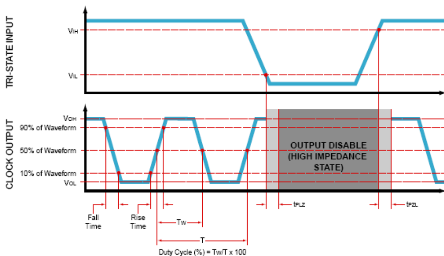
Figure: Tri-State Output Enable / Disable Timing Diagram
