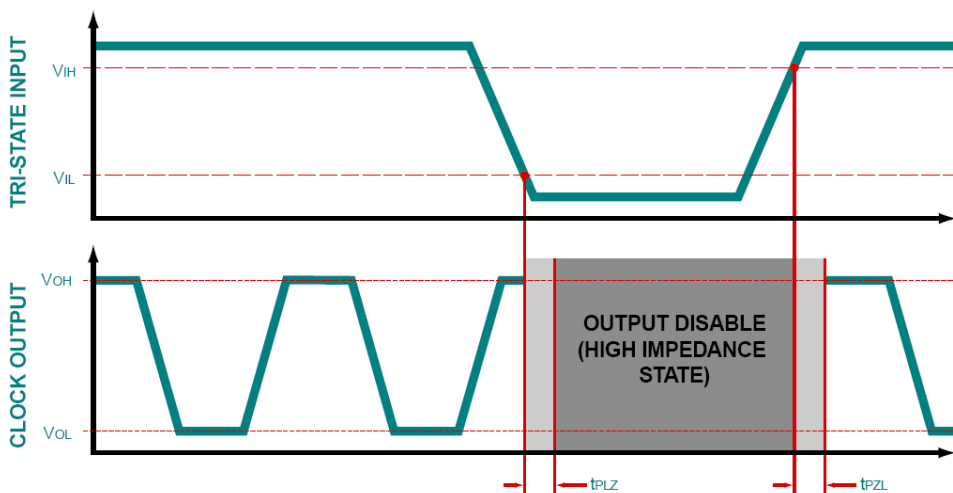
Figure: Tri-State Timing Diagram
